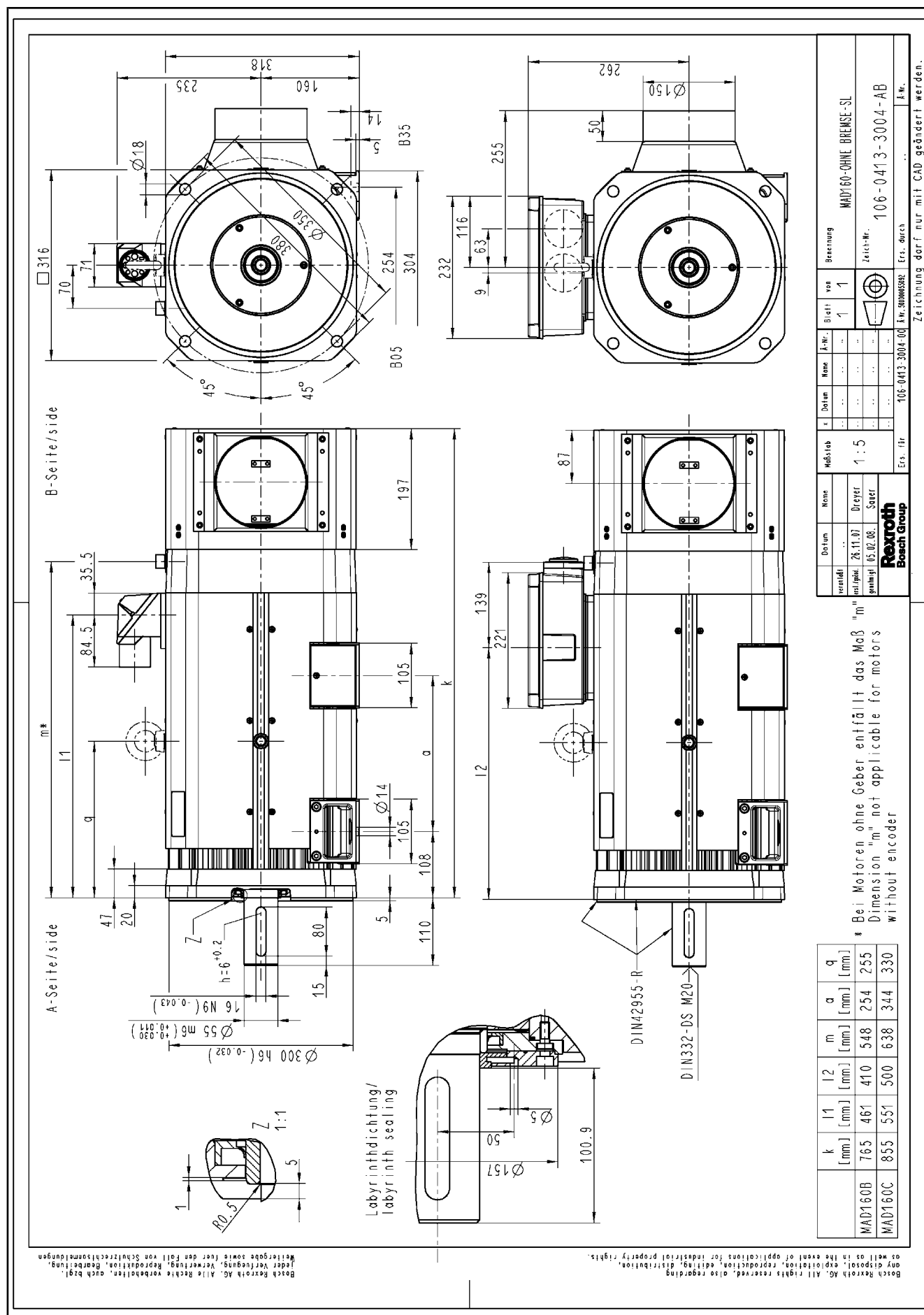
Fig.5-16: MAD160 with SL cooling, without brake
