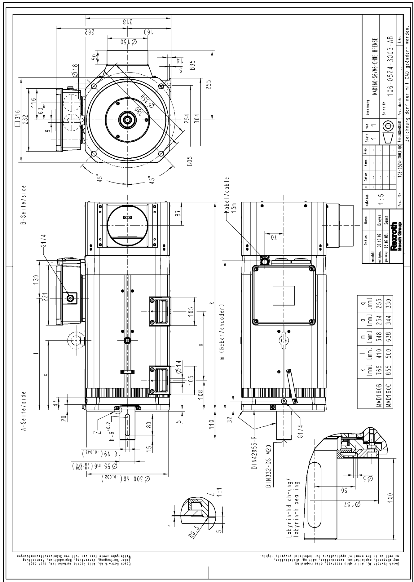
Fig 5-19: MAD160 with M6/S6 encoder, without brake
