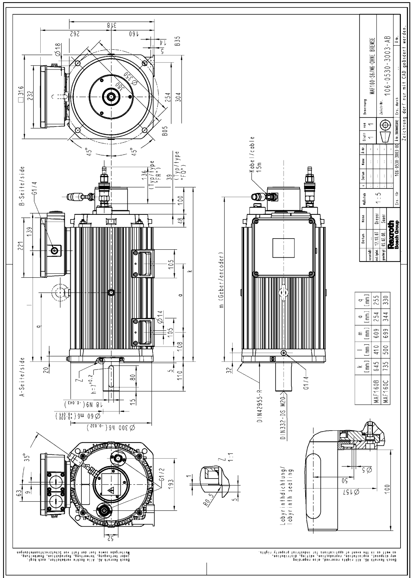
Fig. 5-41: MAF160 with M6/S6 encoder, without brake
