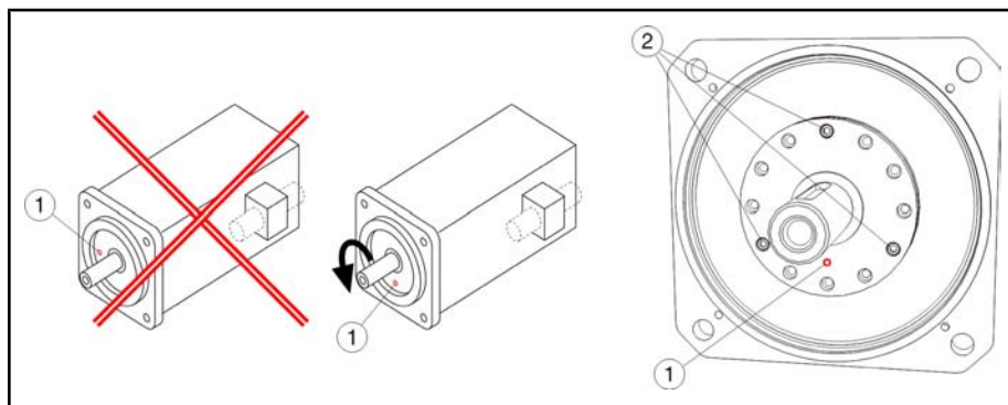
Fig.9-29: Allowed position of the drain hole of the labyrinth seal (example MAD130)
