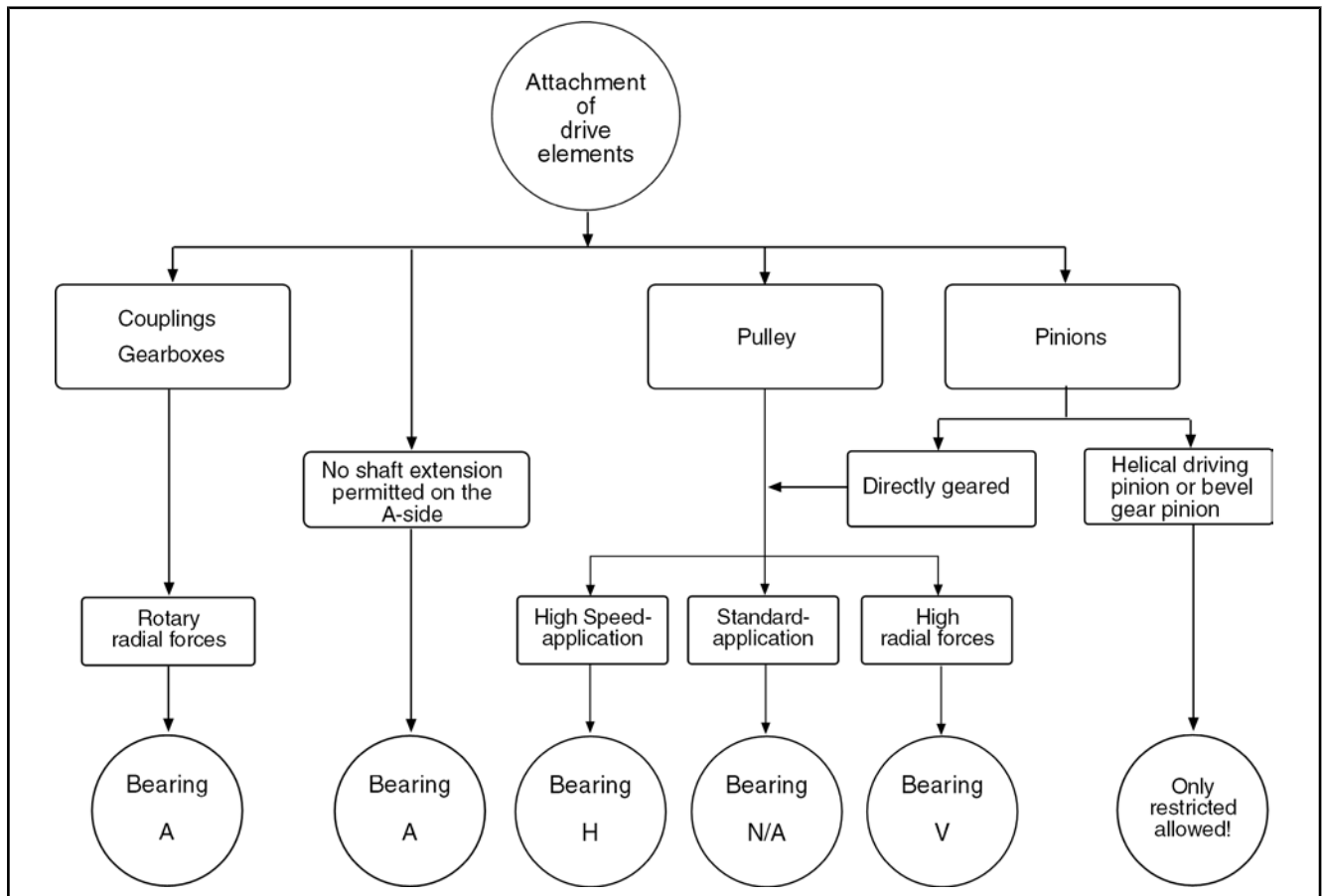
Fig.9-42: Attaching drive elements
